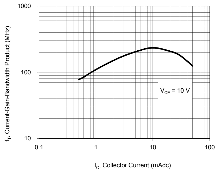
Fig.6 Current-Gain-Bandwidth Product
