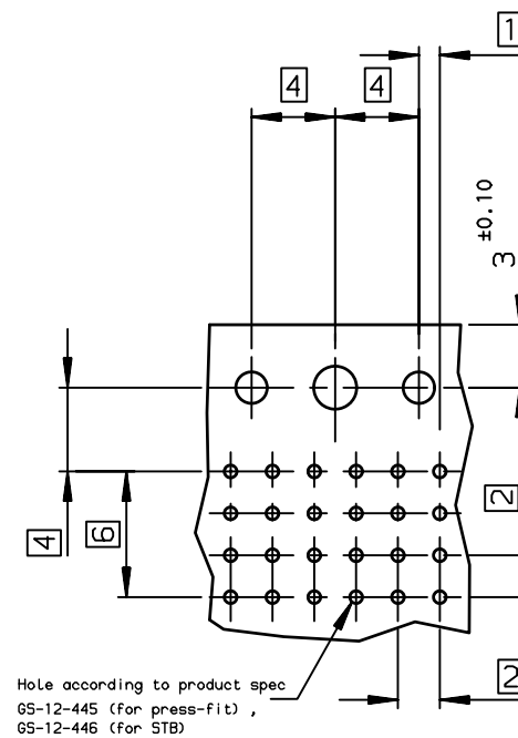
LAYOUT FOR P.C.B (PER 12mm LENGTH)
