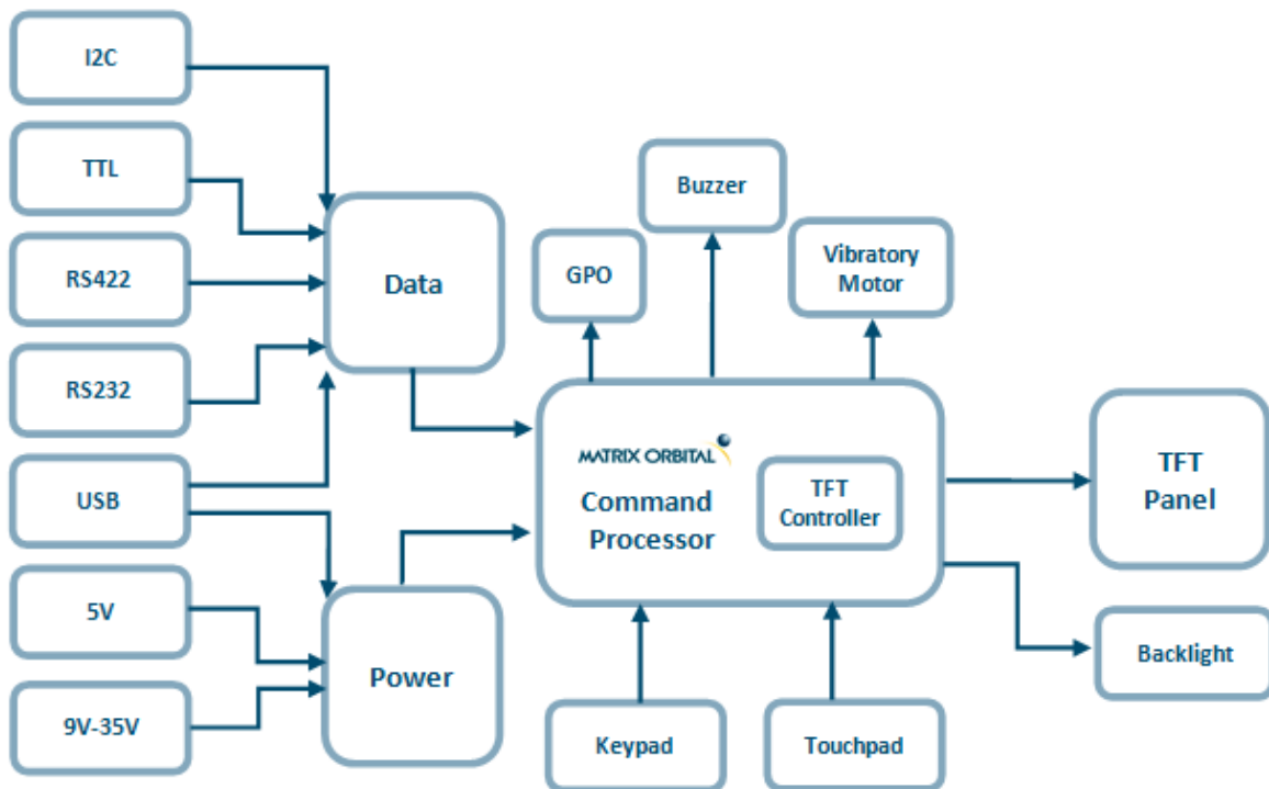
Figure 2: Functional Diagram
