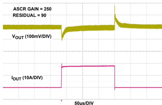
FIGURE 14. 12V_{IN} TO 3.3V_{OUT} TRANSIENT RESPONSE, f_{SW} = 615kHz , C_{OUT} = 3 \times 100\mu F CERAMIC + 2 \times 470\mu F POSCAP
