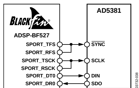
* ADDITIONAL PINS OMITTED FOR CLARITY Figure 38. AD5381-to-ADSP-BF527 Interface
