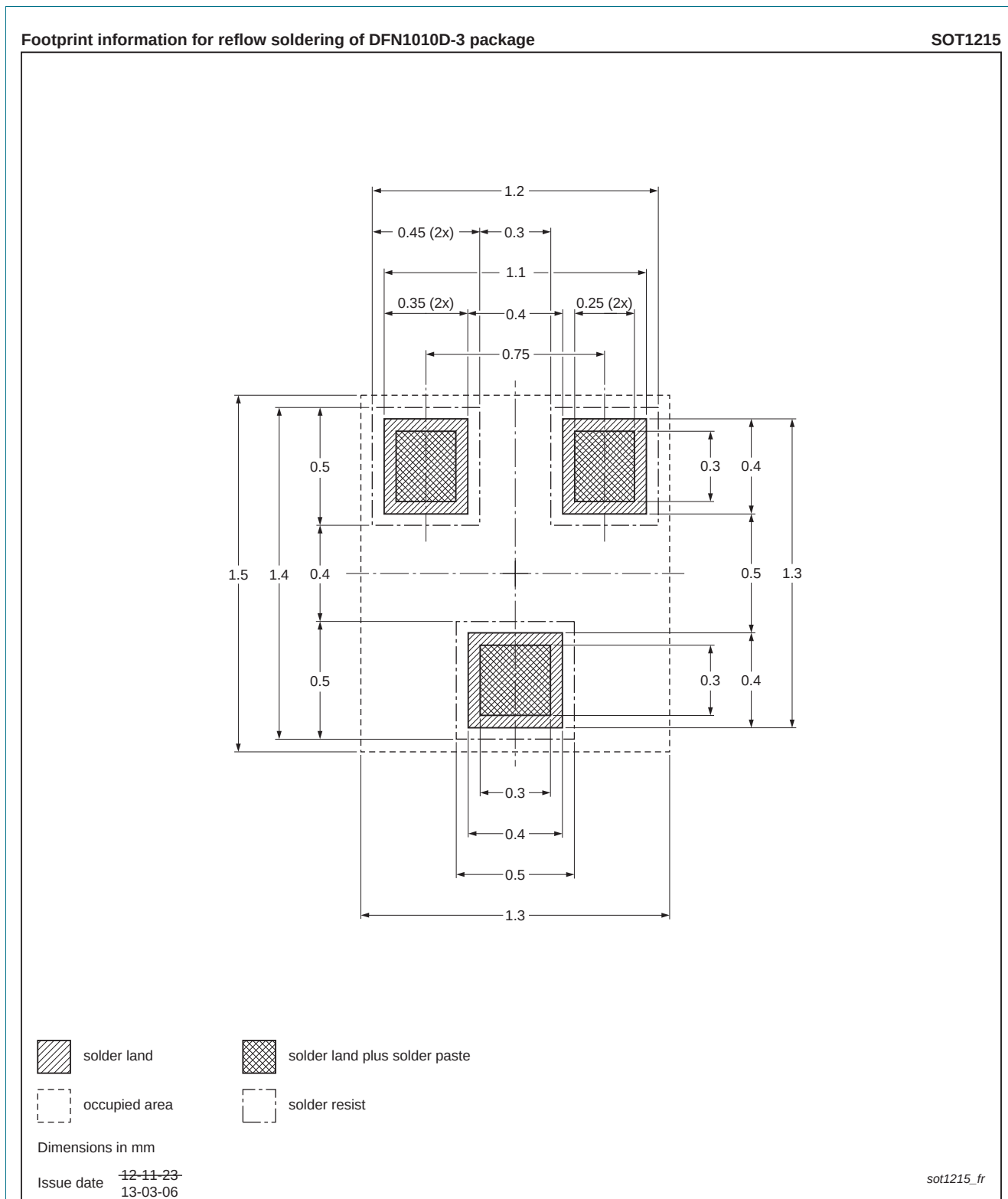
Fig 18. Reflow soldering footprint DFN1010D-3 (SOT1215)
