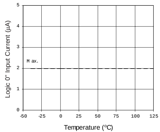
Figure 22A. Logic "0" Input Current vs. Temperature
