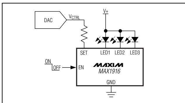
Figure 3. Brightness Adjust Using DAC
