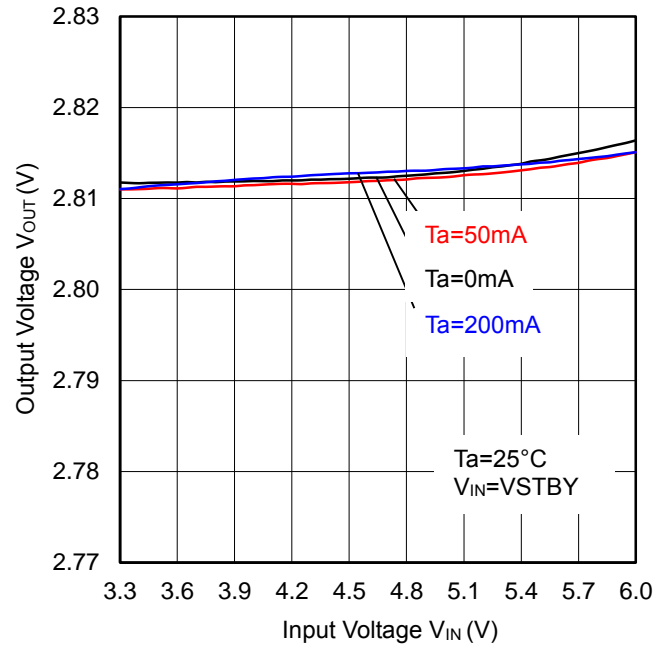
Figure 25. Line Regulation
