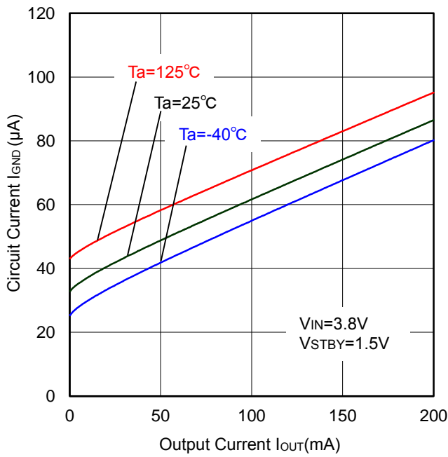
Figure 28. Circuit Current vs. Output Current
