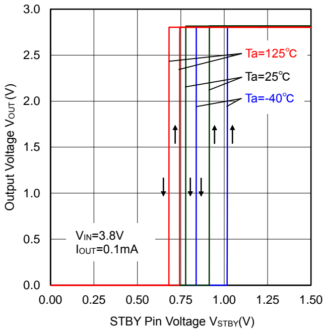
Figure 32. STBY Threshold
