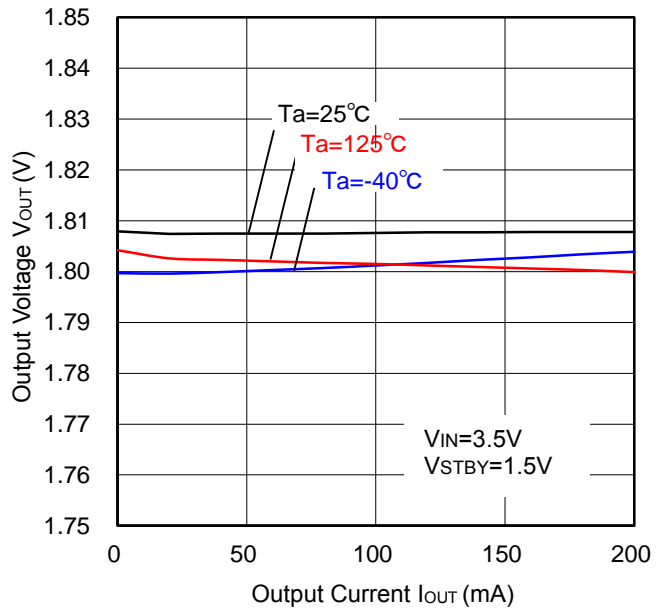
Figure 6. Load Regulation
