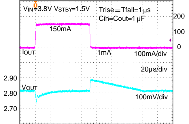
Figure 38. Load Response (1mA to 150mA)
