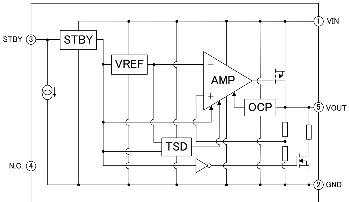
Figure 2. Block diagram
