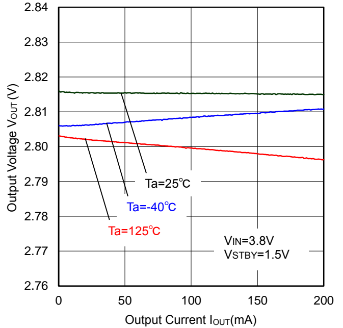
Figure 27. Load Regulation
