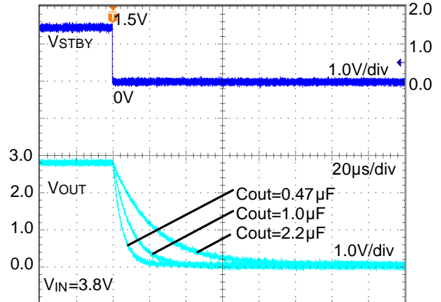
Figure 44. Discharge Time (ROUT=14Ω)
