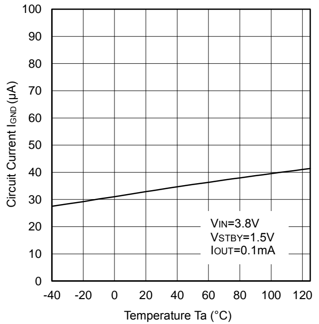
Figure 31. Circuit Current vs. Temperature
