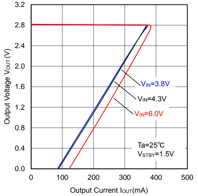
Figure 29. OCP Threshold
