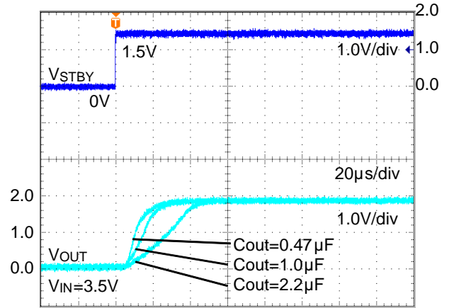
Figure 21. Startup Time (ROUT=9Ω)
