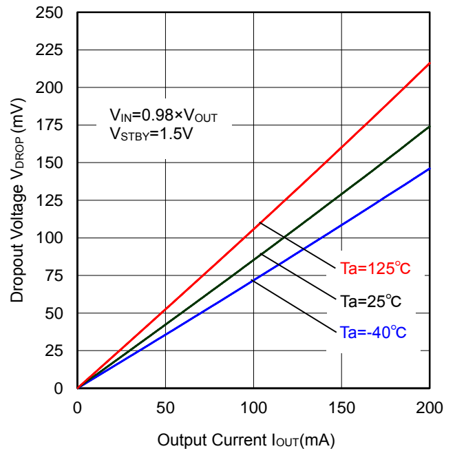
Figure 35. Dropout Voltage vs. Output Current
