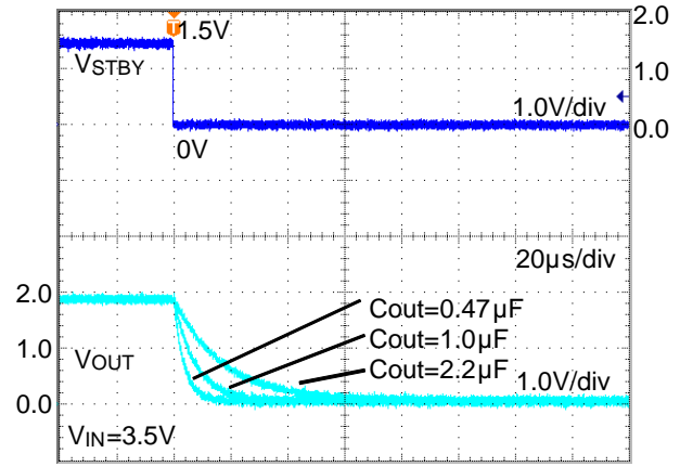
Figure 23. Discharge Time (ROUT=9Ω)
