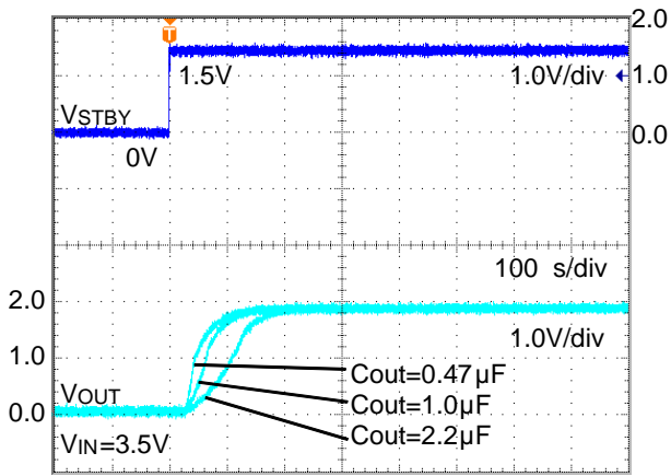
Figure 20. Startup Time (ROUT=open)
