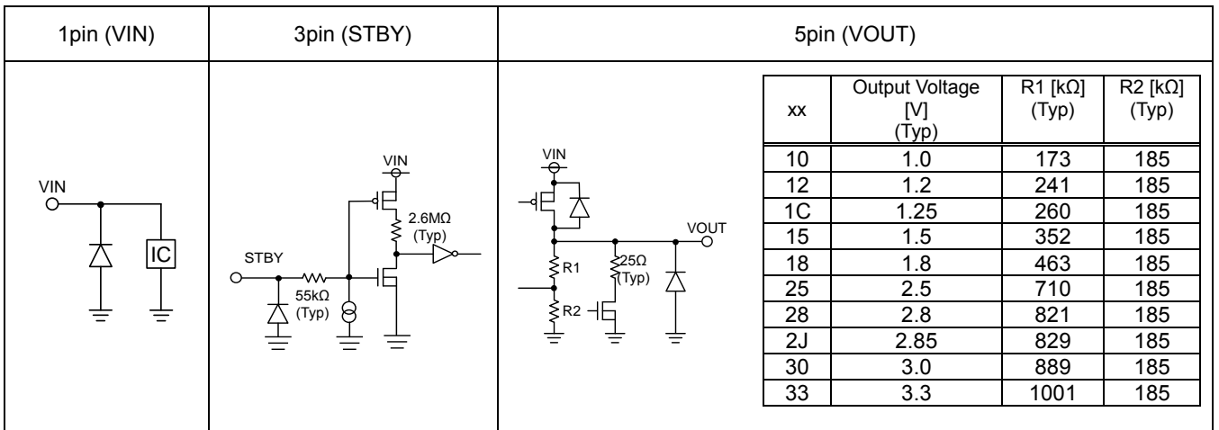
Figure 48. Input / Output equivalent circuit
