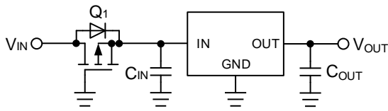
Figure 56. Protection against Reverse Polarity 2
