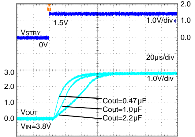
Figure 42. Startup Time (ROUT=14Ω)
