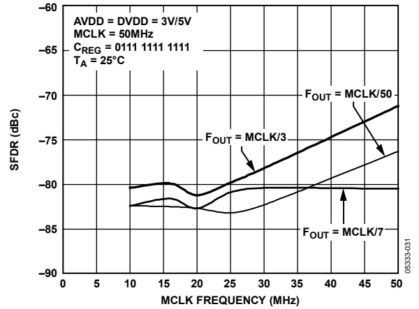
Figure 13. Narrowband SFDR vs. MCLK Frequency
