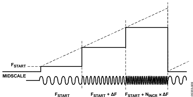
Figure 31. Saw-Sweep Profile
