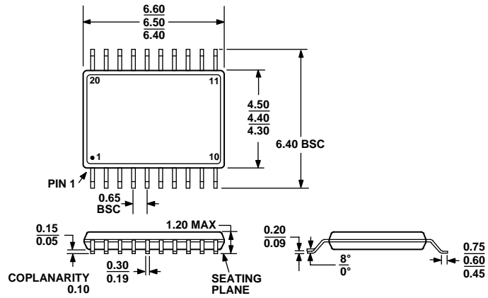
COMPLIANT TO JEDEC STANDARDS MO-153-AC Figure 42. 20-Lead Thin Shrink Small Outline Package (TSSOP) (RU-20) Dimensions shown in millimeters
