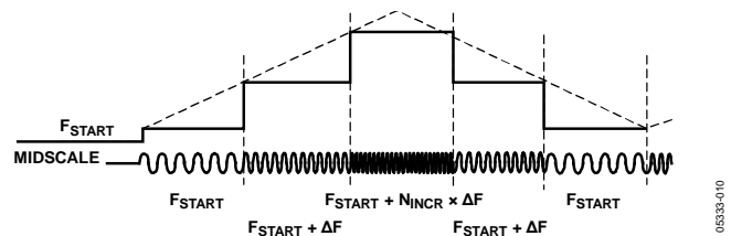
Figure 32. Triangular-Sweep Profile
