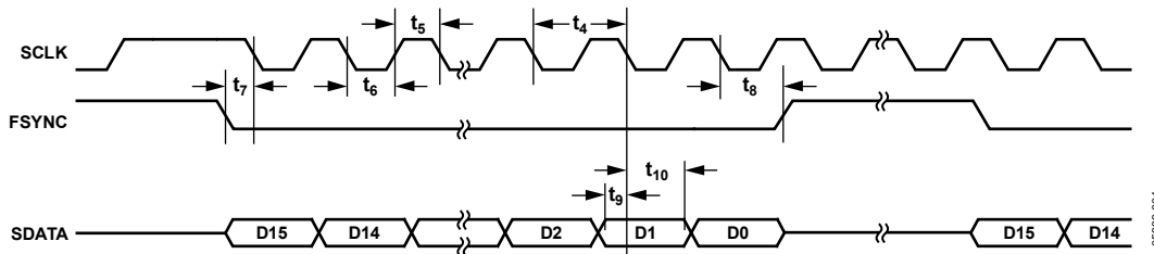
Figure 4. Serial Timing
