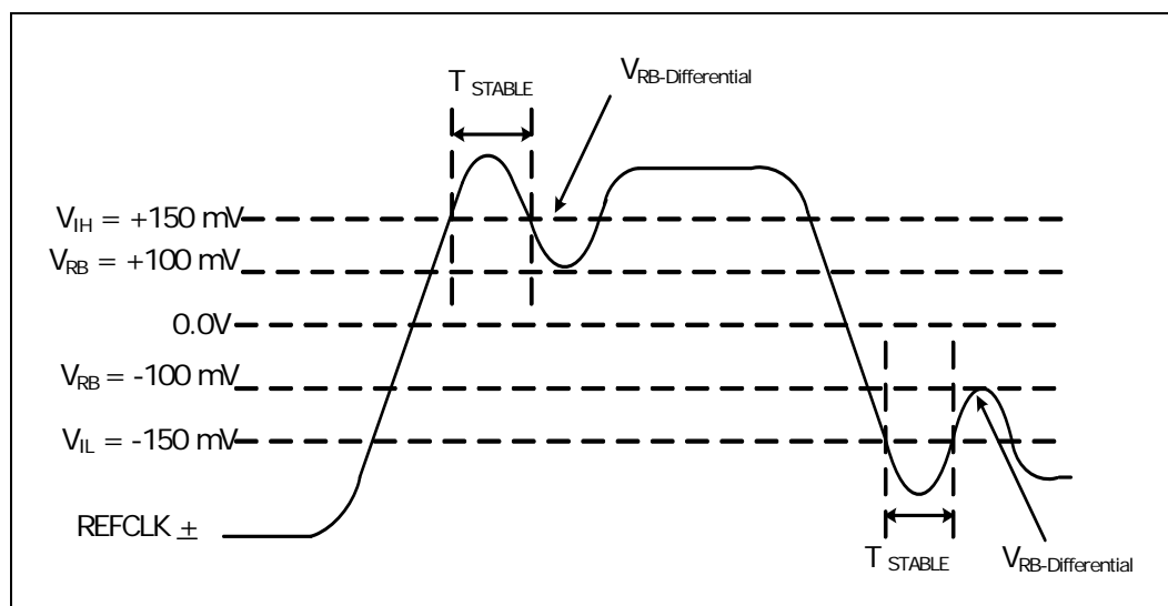
Figure 7-7. BCLK{0/1} Differential Clock Measurement Point for Ringback
