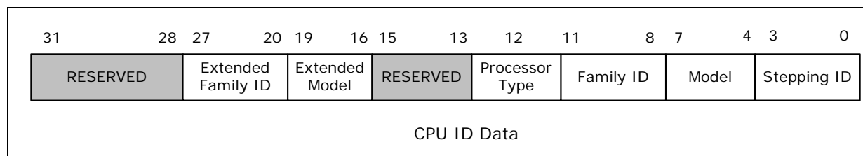
Figure 2-21. CPUID Data
