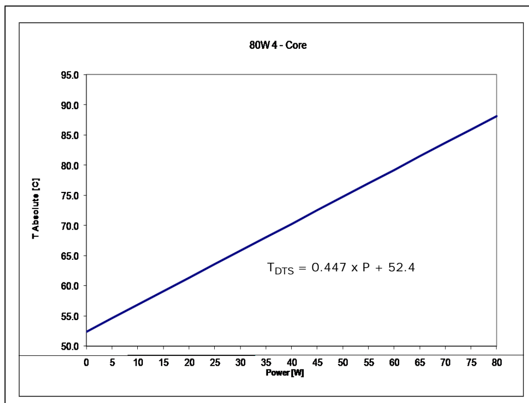
Figure 5-5. Server SKU Platform (4-Core 80W) DTS Based Thermal Profile
