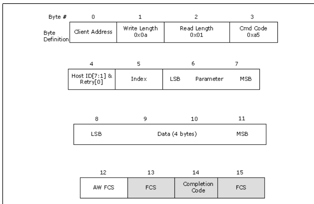
Figure 2-11. WrPkgConfig()
