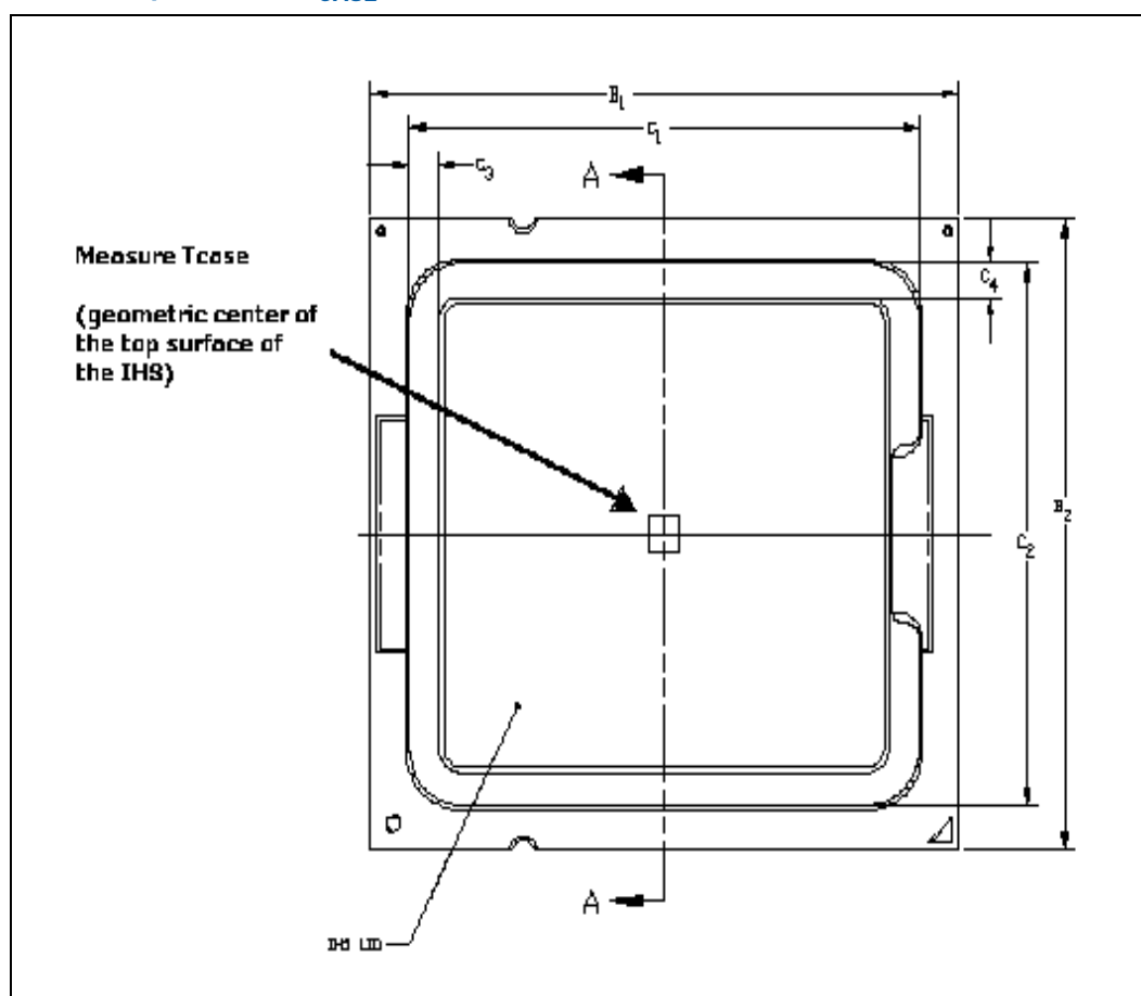
Figure 5-24. Case Temperature ( T_{CASE} ) Measurement Location
