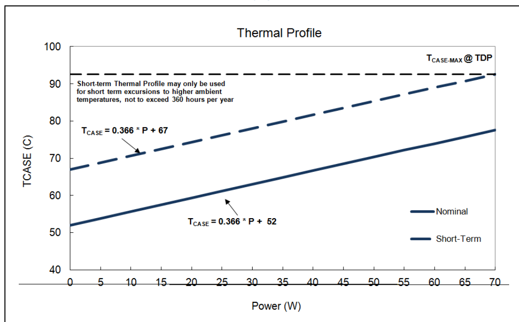
Figure 5-16. Embedded Server SKU (LV70W-8C) T_{CASE} Thermal Profile
