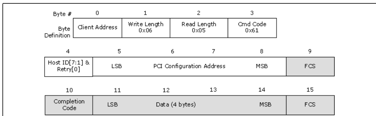
Figure 2-45. RdPCISig()
