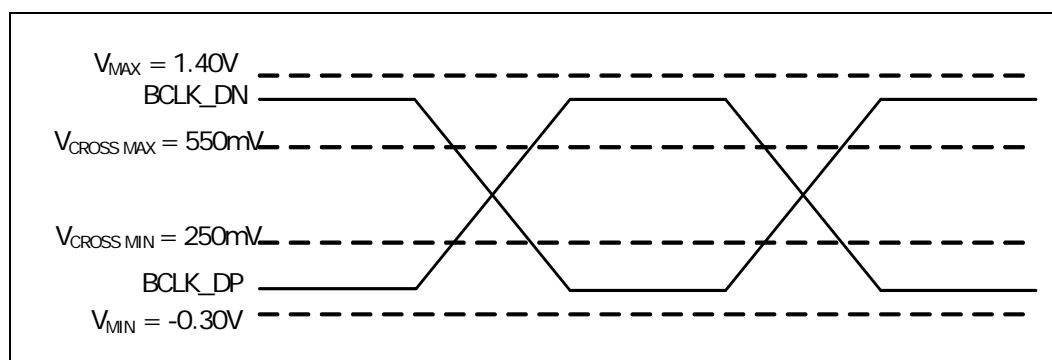
Figure 7-8. BCLK{0/1} Single Ended Clock Measurement Points for Absolute Cross Point and Swing
