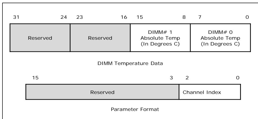
Figure 2-14. Intel® Xeon® Processor E5-2400 Product Families DIMM Temperature Read / Write
