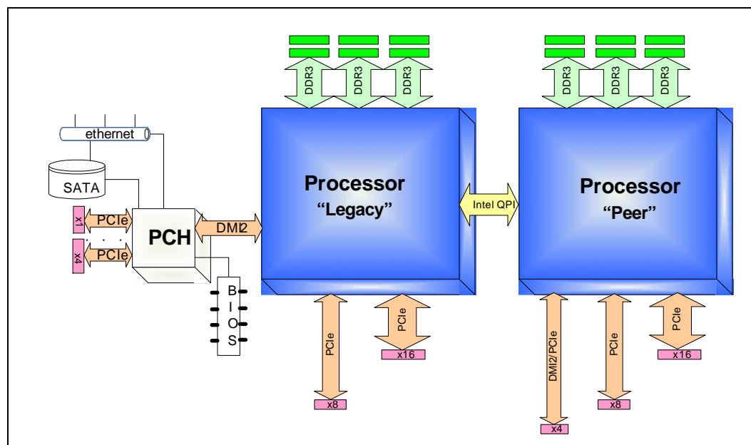
Figure 1-1. Intel® Xeon® Processor E5-2400 Product Family on the 2 Socket Platform
