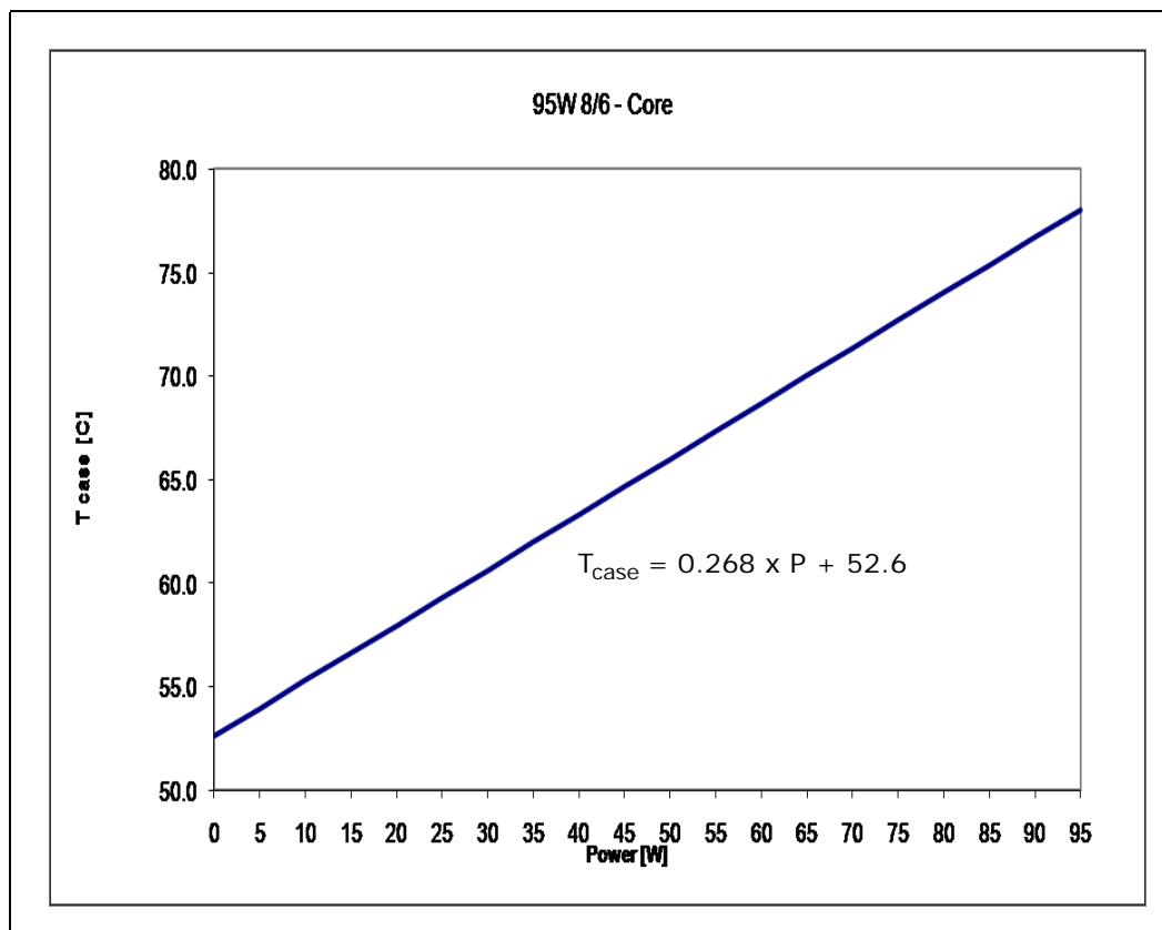
Figure 5-1. Server SKU Platform (8-Core / 6-Core 95W) T CASE Thermal Profile
