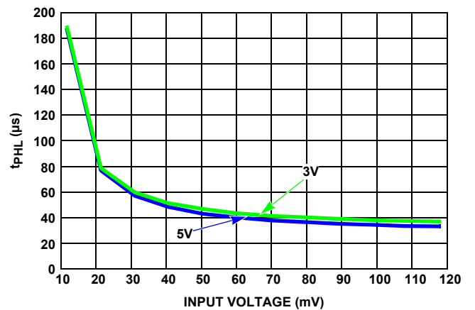
FIGURE 23. OUTPUT RESPONSE TIME vs INPUT OVERDRIVE (t PHL )
