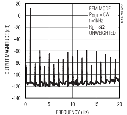
OUTPUT FREQUENCY SPECTRUM
