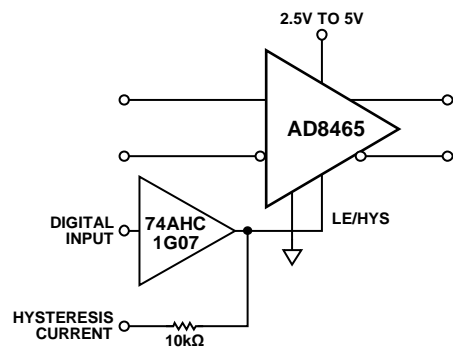
Figure 25. Hysteresis Adjustment with Latch
