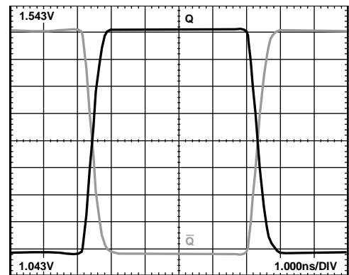
Figure 15. 50 MHz Output Voltage Waveform at V_{CCO} = 5.5 V
