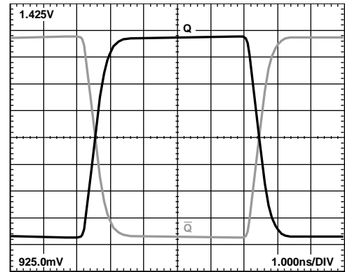
Figure 14. 50 MHz Output Voltage Waveform at V_{CCO} = 2.5 V
