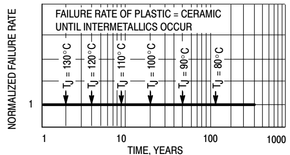
Figure 3. Failure Rate vs. Time Junction Temperature
