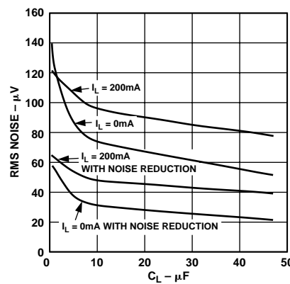
Figure 18. RMS Noise vs. C_L (10 Hz-100 kHz)
