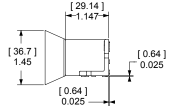
Receptacle Outline
