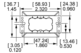
Receptacle Outline
