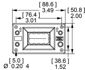
Plug Outline
