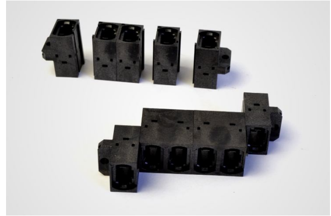
MPO Straight End Ear Adapters
