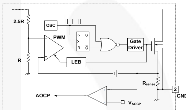
Figure 35. AOCB Block
