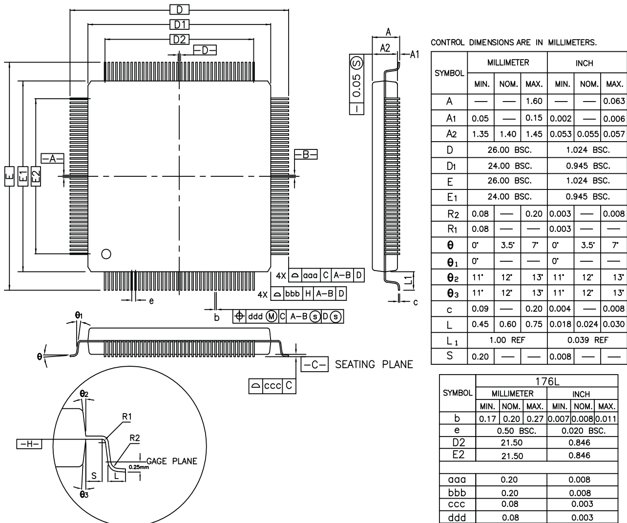
Figure 46-1. 176-lead LQFP Package Drawing
