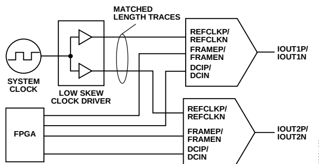
Figure 62. Typical Circuit Diagram for Synchronizing Devices
