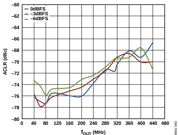
Figure 16. Four-Carrier W-CDMA ACLR vs. f_{OUT} over Digital Scale, Adjacent Channel, 4x Interpolation, f_{DATA} = 245.76 MSPS, PLL Off
