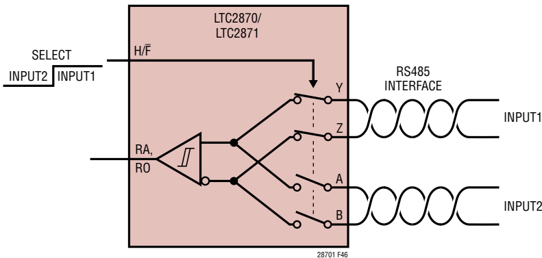
Figure 49. RS485 Receiver with Multiplexed Inputs
