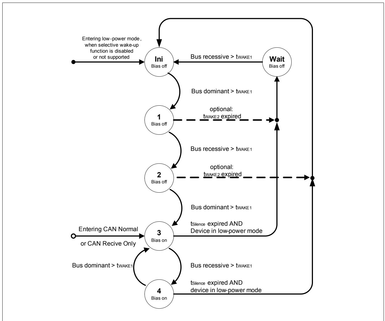
Figure 22 WUP detection following the definition in ISO 11898-5
