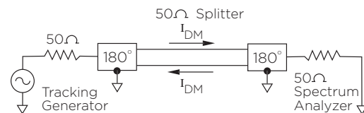
Reference Connection
