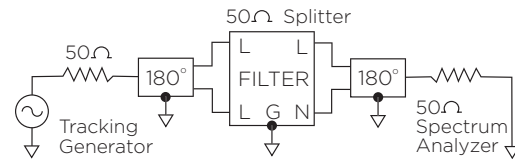
Test Connection
