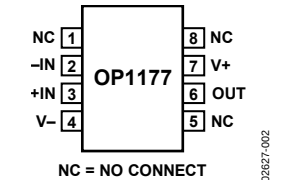
Figure 2. 8-Lead SOIC_N (R Suffix)
