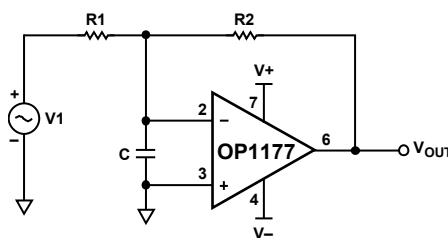
Figure 61. EMI Reduction
