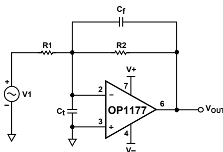
Figure 60. Compensation Using Feedback Capacitor
