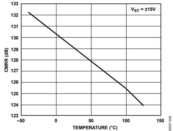
Figure 28. CMRR vs. Temperature
