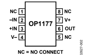
Figure 2. 8-Lead SOIC_N (R Suffix)
