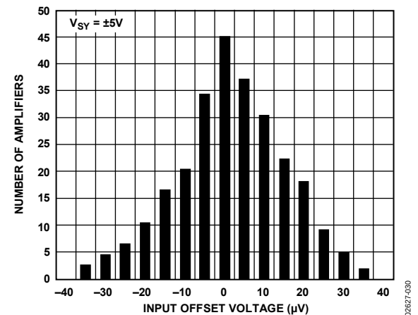
Figure 30. Input Offset Voltage Distribution
