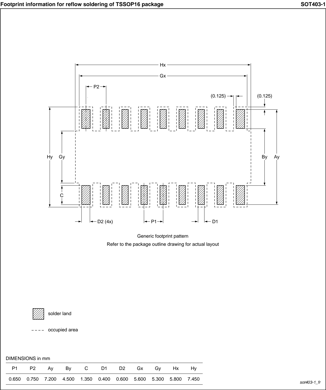
Fig 15. PCB footprint for SOT403-1 (TSSOP16); reflow soldering
