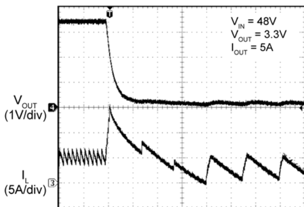
Short Circuit
