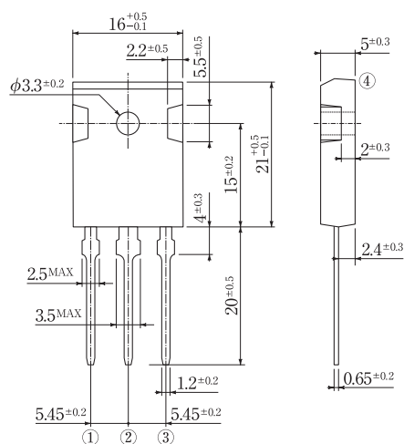
Fig.46 Package: MTO-3P
