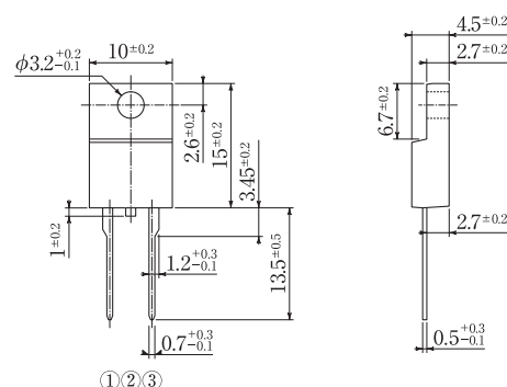
Fig.49 Package: FTO-220A
