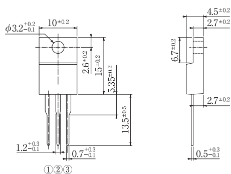
Fig.48 Package: FTO-220
