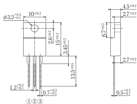
Fig.50 Package: FTO-220A
