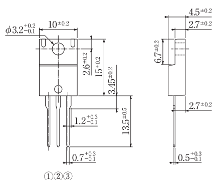
Fig.52 Package: FTO-220G
