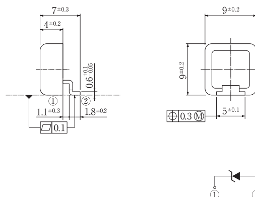
Fig.80 Package: MCP
