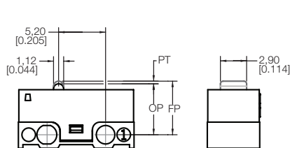
TYPE A PIN PLUNGER
