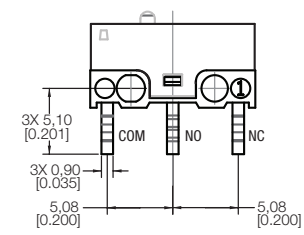
TYPE 30 - PCB SNAP-IN
