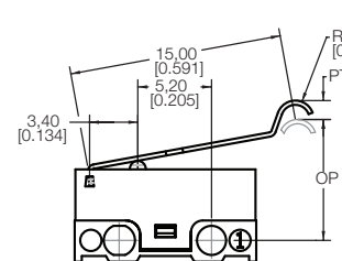
TYPE H SIMULATED ROLLER LEVER (15,0 mm; R1.3)
