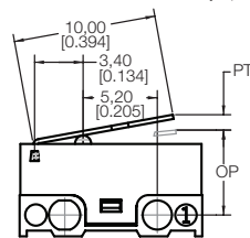
TYPE B SHORT STRAIGHT LEVER (10,0 mm)
