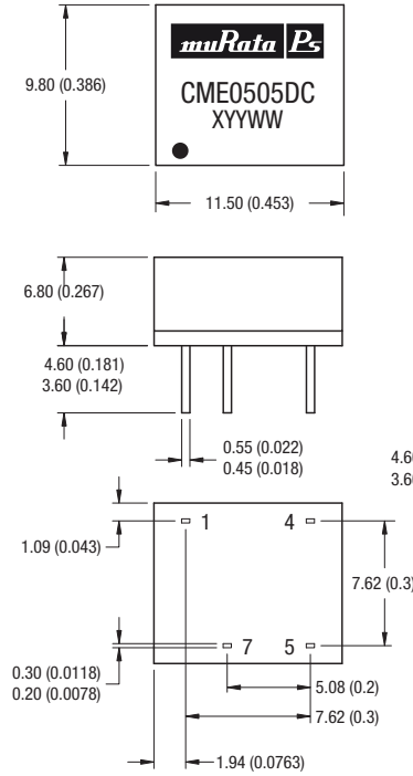
DC Package
