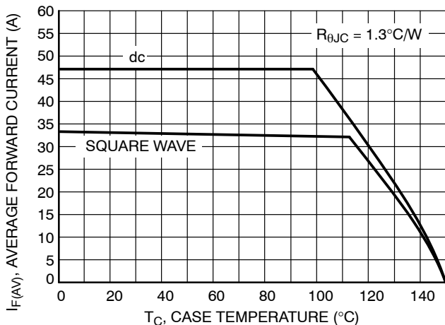
Figure 5. Current Derating
