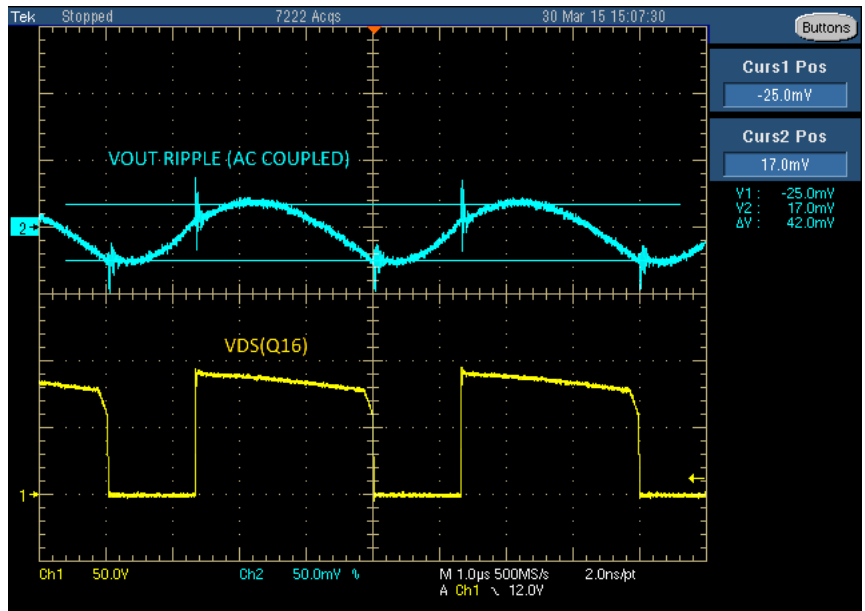
Figure 5. Output Voltage Ripple ( V_{PORT} = 57V, 5V/13A )
