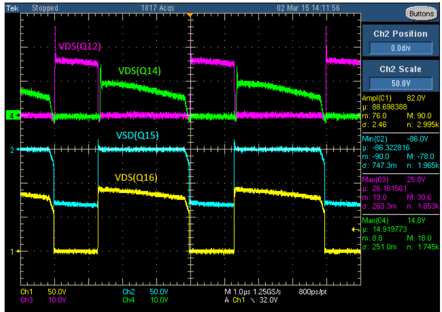
Figure 4. Stresses ( V_{PORT} = 57V, 5V/13A )
