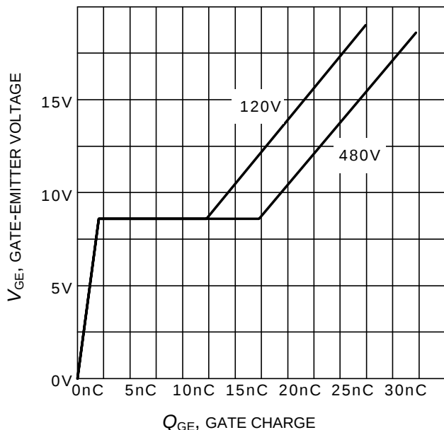
Figure 17. Typical gate charge ( I_C=4A )
