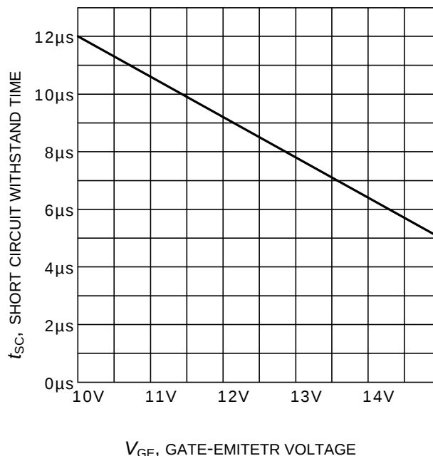
Figure 20. Short circuit withstand time as a function of gate-emitter voltage ( V_{CE}=400V , start at T_j=25^\circ C , T_{jmax}<150^\circ C )
