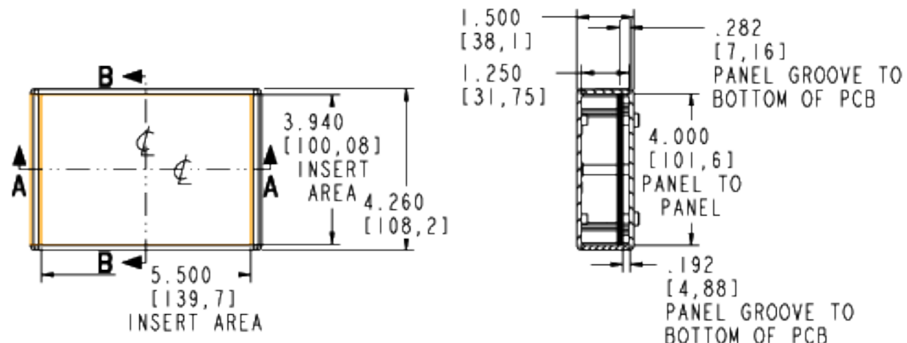
SECTION B-B
