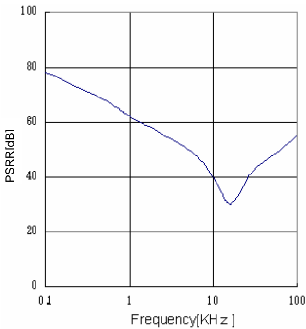
Fig.20 PSRR ( I_o=0mA )
