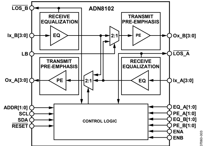
Figure 38. Simplified Functional Block Diagram
