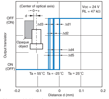
Fig 4. Repeated Sensing Position Characteristics
