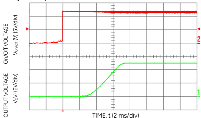
Figure 14. Typical Start-Up Using Remote On/Off ( V_{in} = 12.0 Vdc, V_o = 5.0 Vdc, I_o = 10.0 A).
