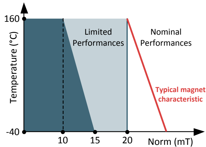
fig. 10 - Minimum useful signal definition for Standard/Legacy application
