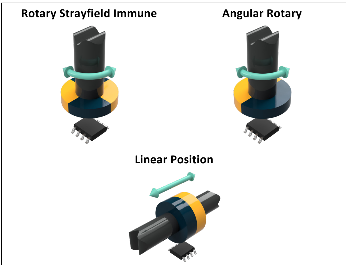
fig. 2 - Application Modes
