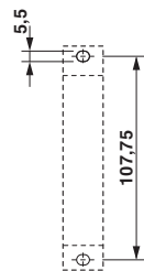
Dimensional drawing
