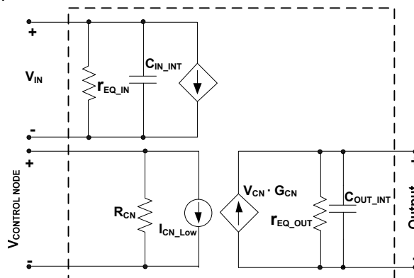
Figure 24 – PRM48A[x]480[y]400A00 AC small signal model
