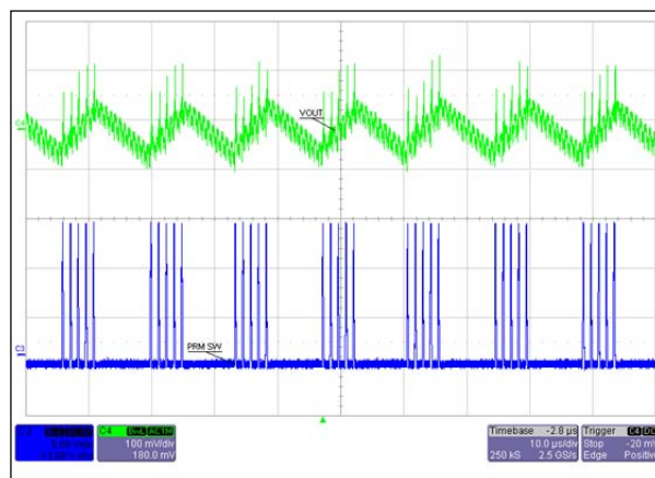
Figure 39 – light load burst mode of operation
