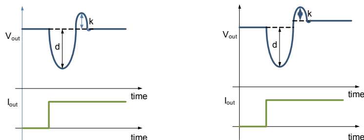
(a) without Adaptive Loop (b) with Adaptive Loop Figure 38 – load step response example and “droop” vs. “kick” definition. (a) with Adaptive Loop; (b) without Adaptive Loop.
