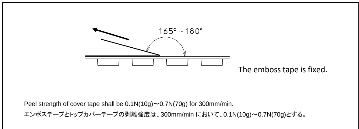
Figure 5-6 Peel Strength
