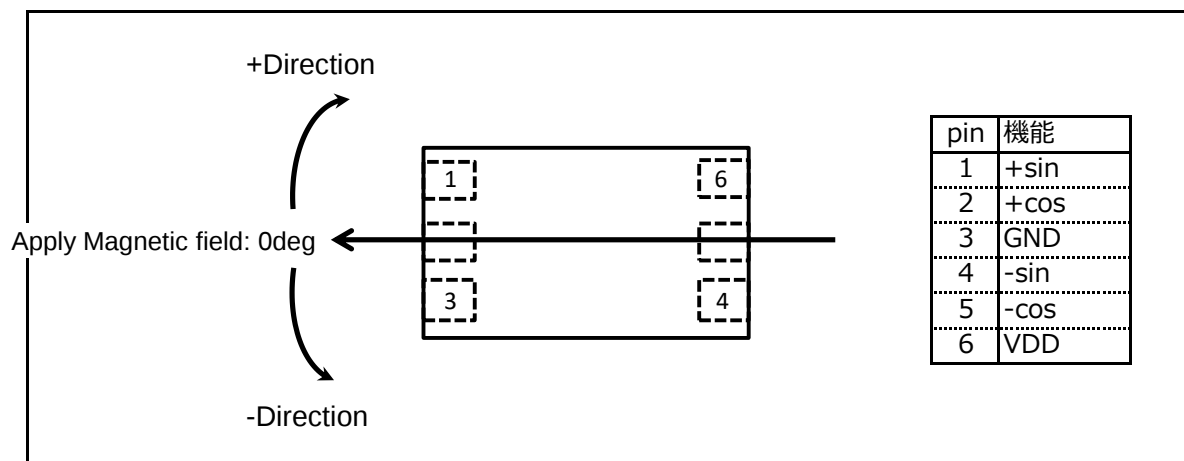
Figure 3-1 Definition of Magnetic Field Direction
