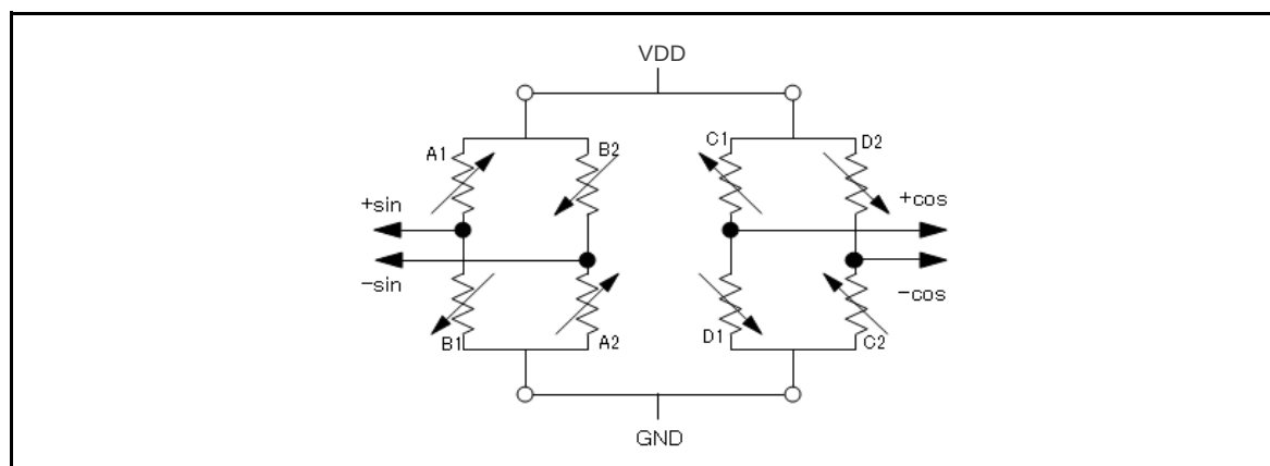
Figure 3-2 Equivalent Circuit
