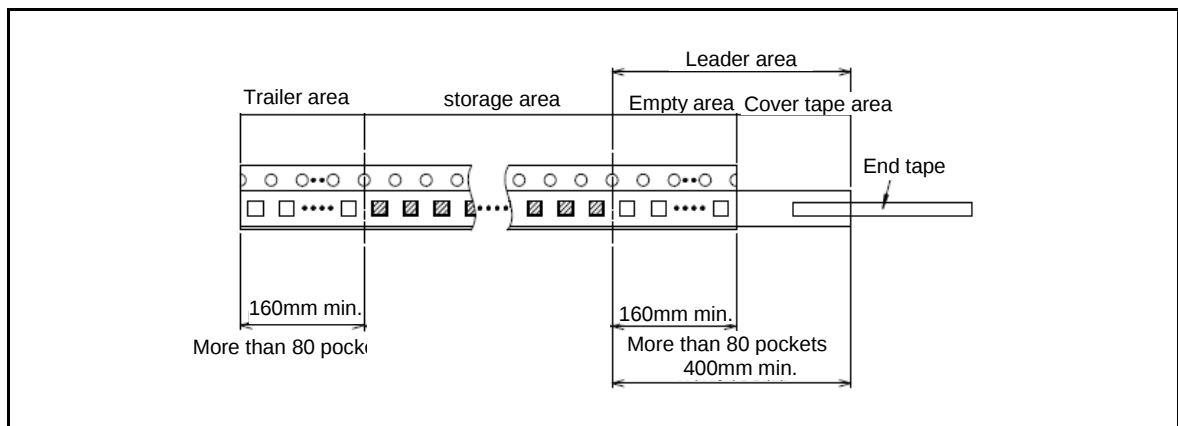
Figure 5-5 Taping Specification
